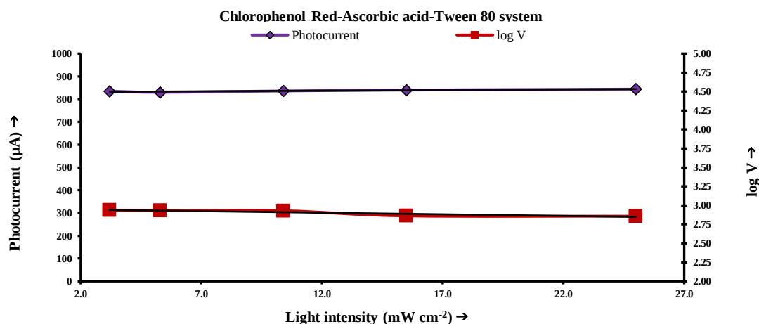
Fig. 1 Variation of photocurrent and log V with light intensity
