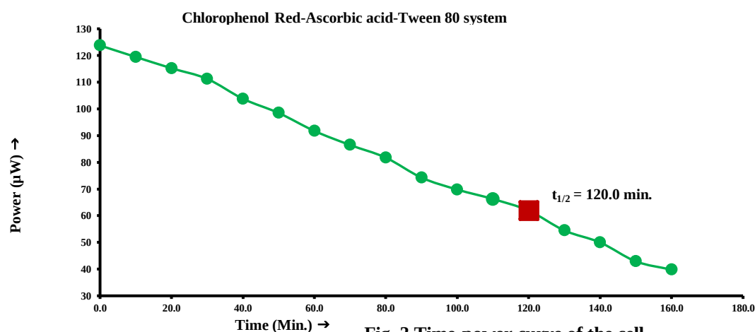
Fig. 3 Time-power curve of the cell
