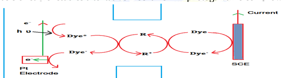
Fig. 4 Scheme of mechanism
