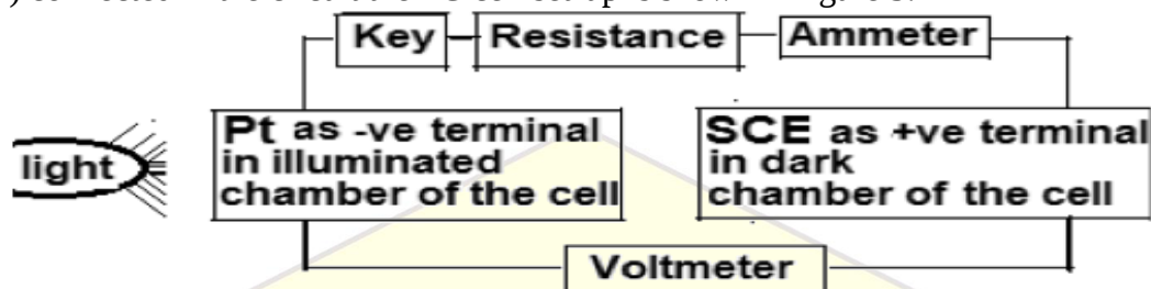
Fig.5 Photogalvanic Cell Set-up
