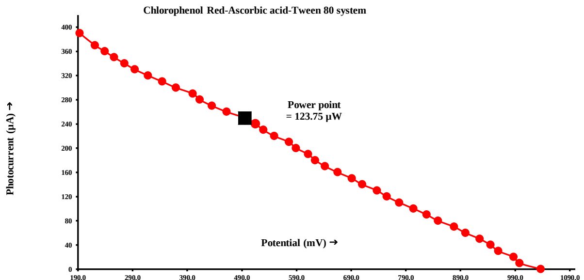
Fig. 2 current voltage properties (i-V) of the photogalvanic cell
