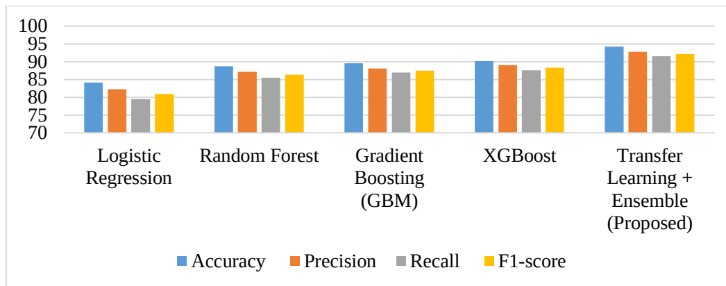
Figure 1: Graphical Representation of Performance Metrics of Different Models
