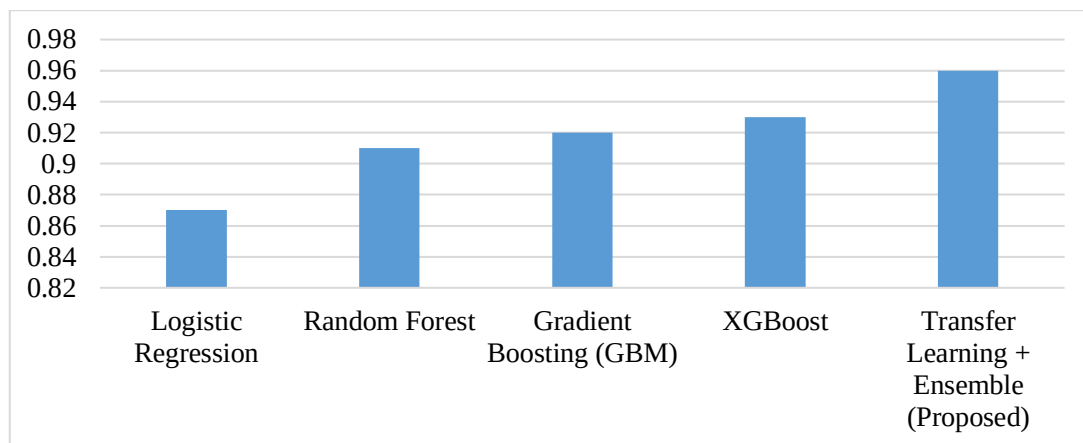
Figure 3: Graphical Representation of AUC-ROC Comparison Across Models
