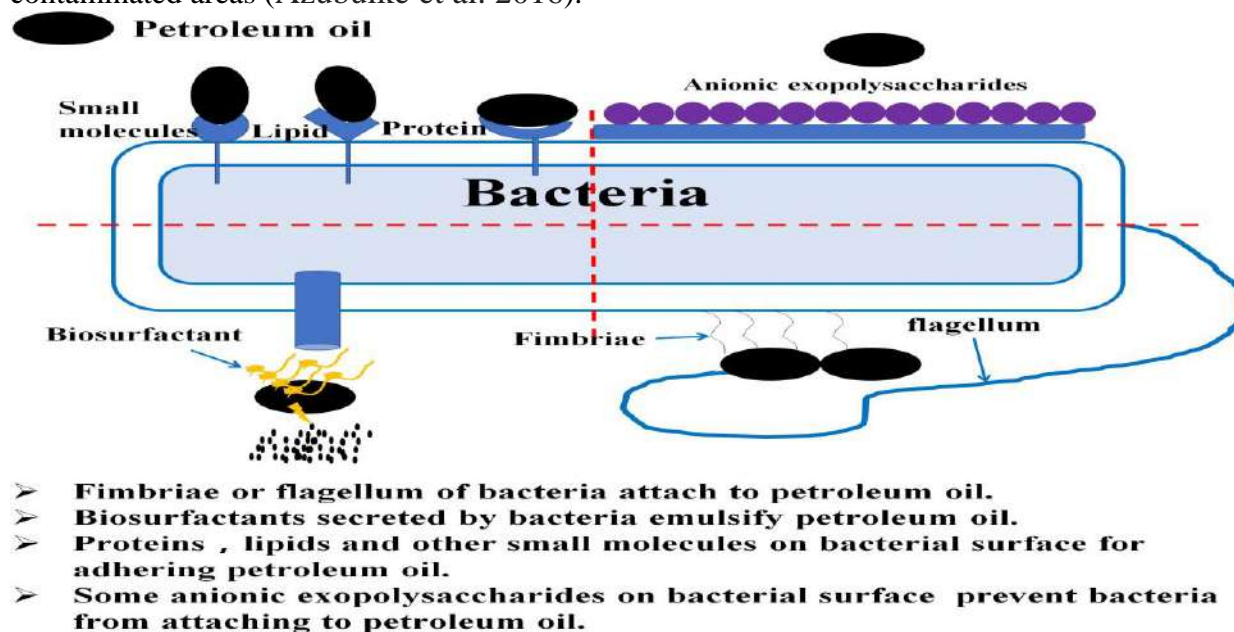
Figure 2. Schematic representation of the interaction between bacteria and petroleum hydrocarbons (Xu et al. 2018).
