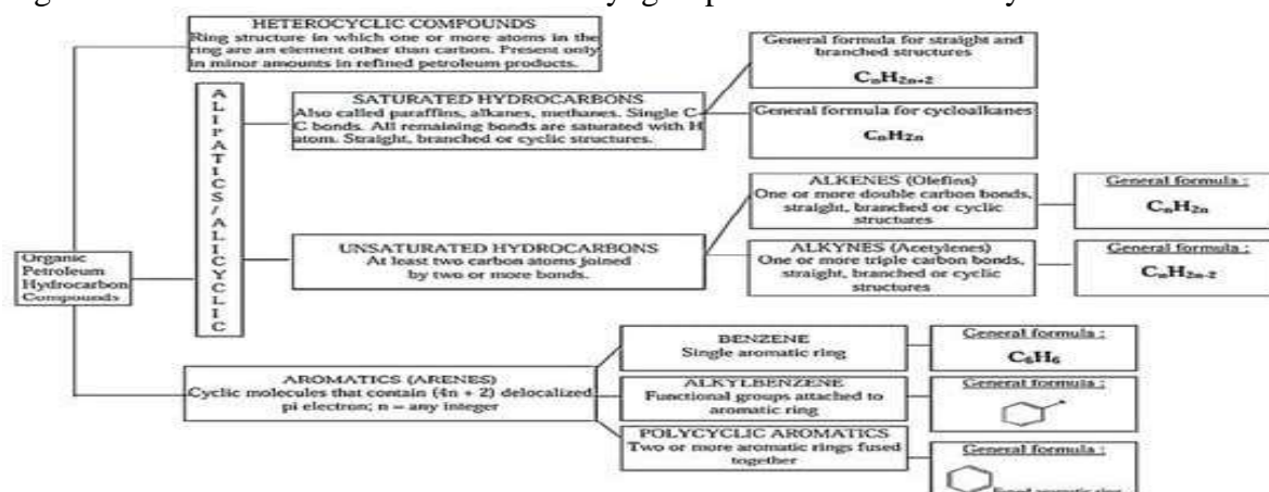
Figure 1. A list of the many categories and subcategories of all petroleum hydrocarbons (Hidayat and Turjaman 2016).
