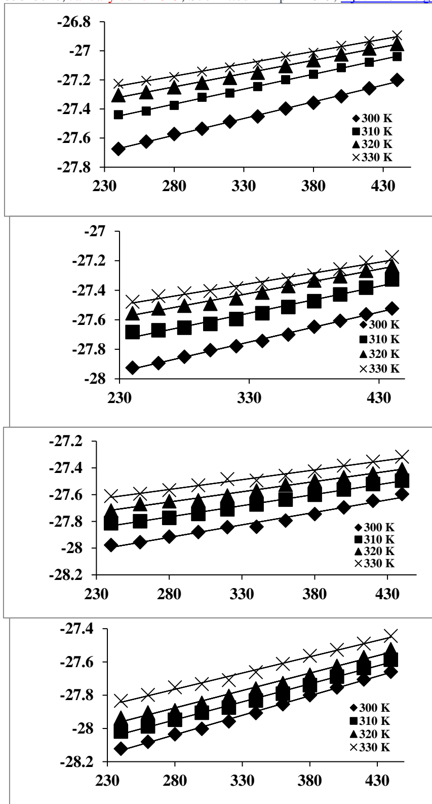
Fig. 2. \ln(I/V) vs. V in thin-films of a\text{-Se}_{90}\text{Sb}_6\text{Ag}_4 before and after illumination of white light at (a) 0 hour, (b) 2 hours, (c) 4 hours, (d) 6 hours.
