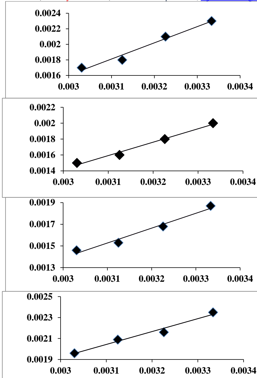
Fig. 3. Slope (S) vs. 1/T in thin-films of a\text{-Se}_{90}\text{Sb}_6\text{Ag}_4 before and after prolonged illumination of white light at (a) 0 hour, (b) 2 hours, (c) 4 hours, (d) 6 hours.
