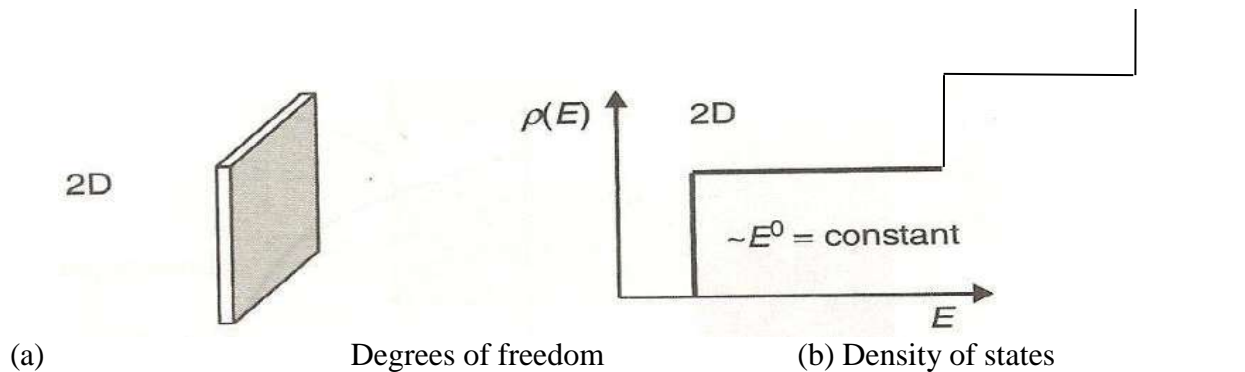
Figure: 1.2 (a) Electron trapped in 2D plane: Quantum well. (b) The DOS variation of quantum well as a function of energy. DOS(2D) shows a step function behaviour.
